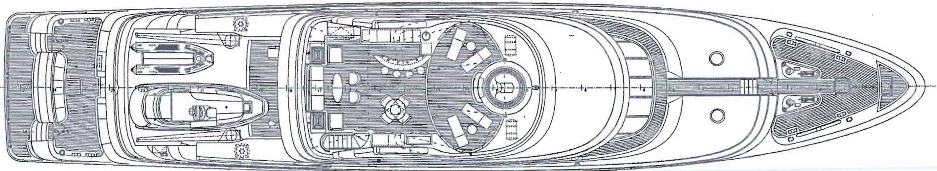
SUN DECK
