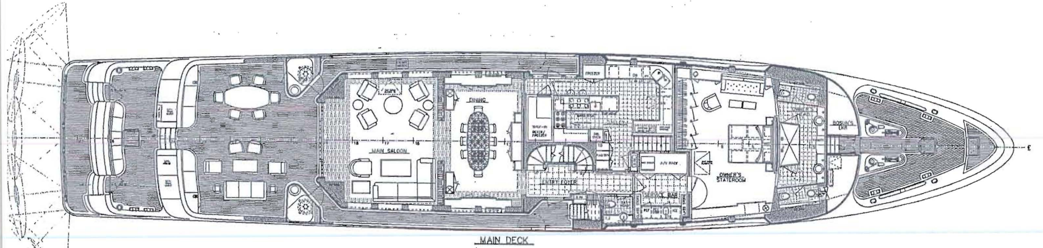
MAIN DECK
