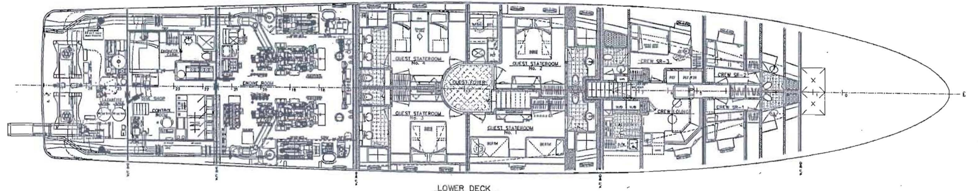
LOWER DECK
