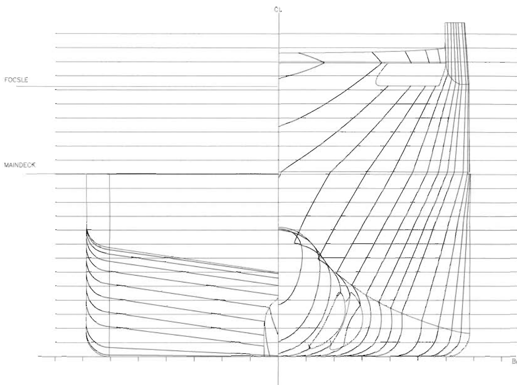
Figure 5: Body Plan Lines
