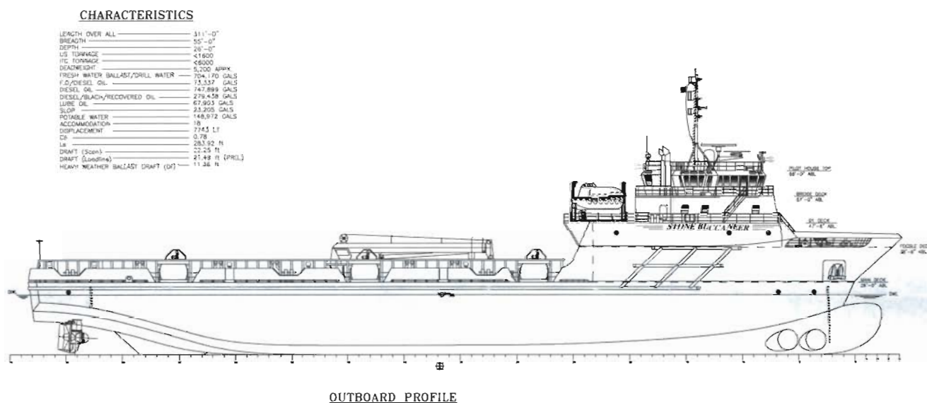
OUTBOARD PROFILE
